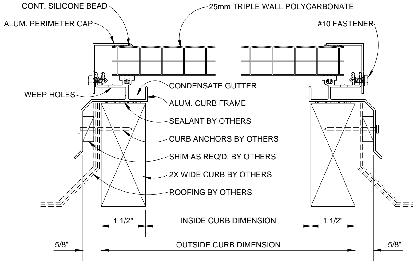
MODEL: A-S-CM-25mm HALF SCALE
