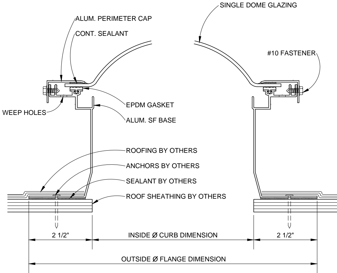
MODEL: A-C-SF1 HALF SCALE
